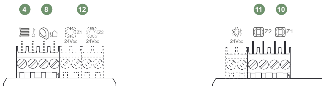
fig. 14 - Raccordements Sondes
