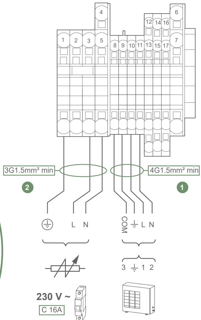
fig. 12 - Raccordements Alimentations
