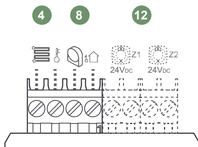
fig. 16 - Raccordements Sondes
